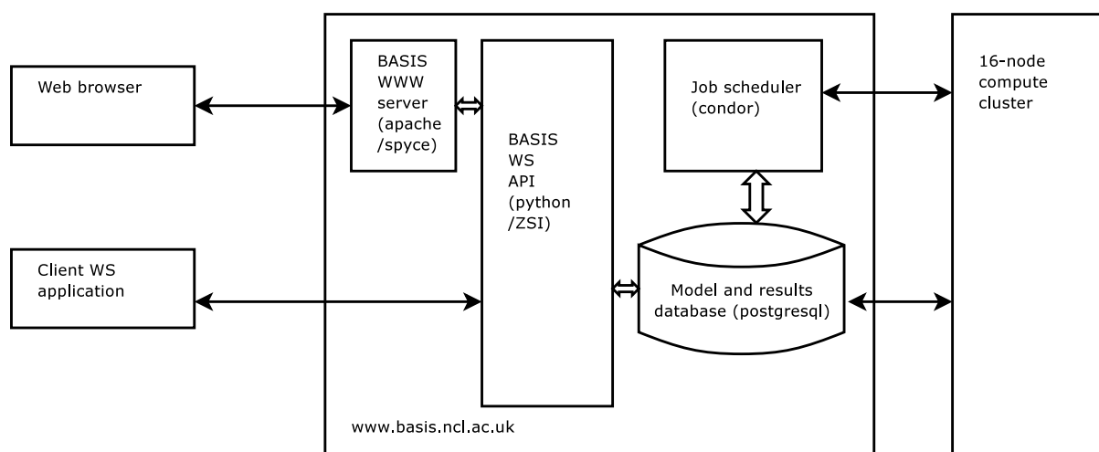
Figure 2: BASIS Architecture
